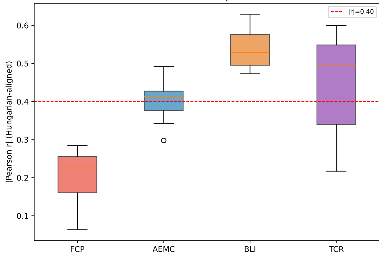
Route 3: VAE seed stability across 10 seeds
