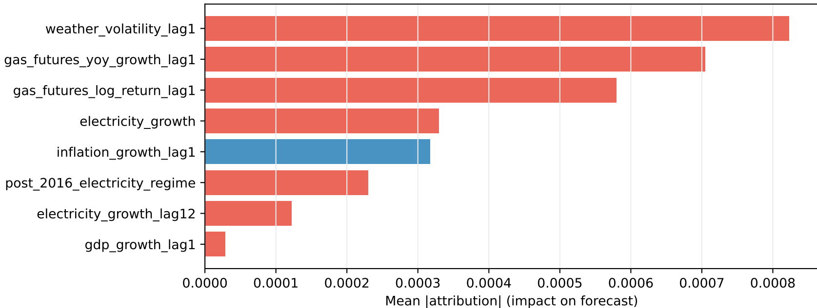
LSTM — Gradient×Input Attribution Electricity 2017 (mean over lookback)
