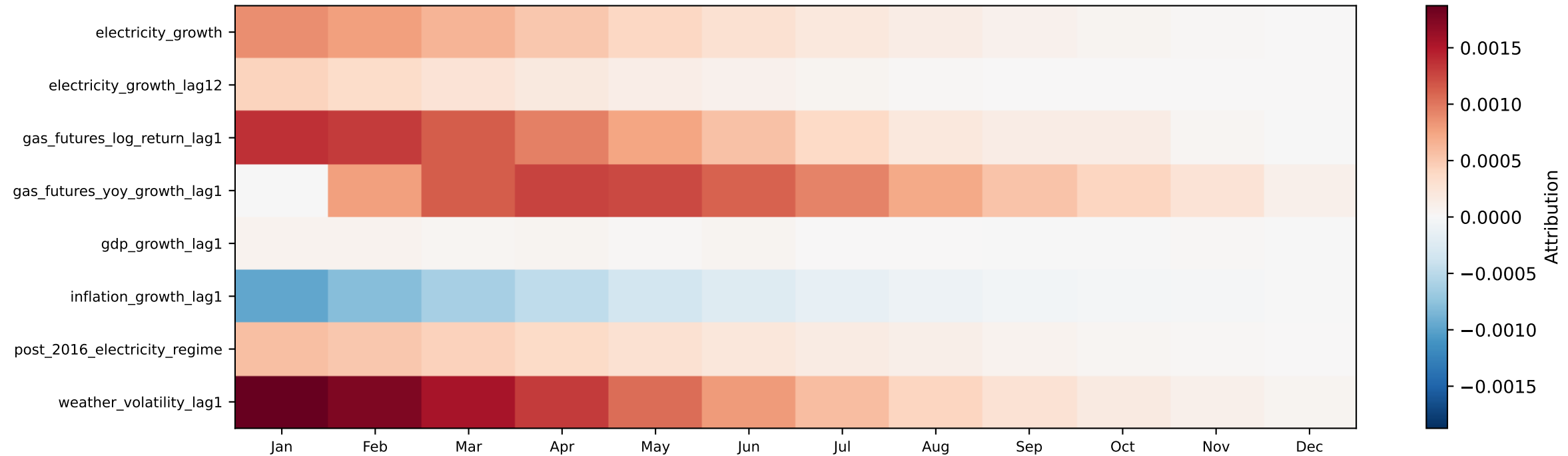
LSTM Attribution Heatmap — Electricity 2017
