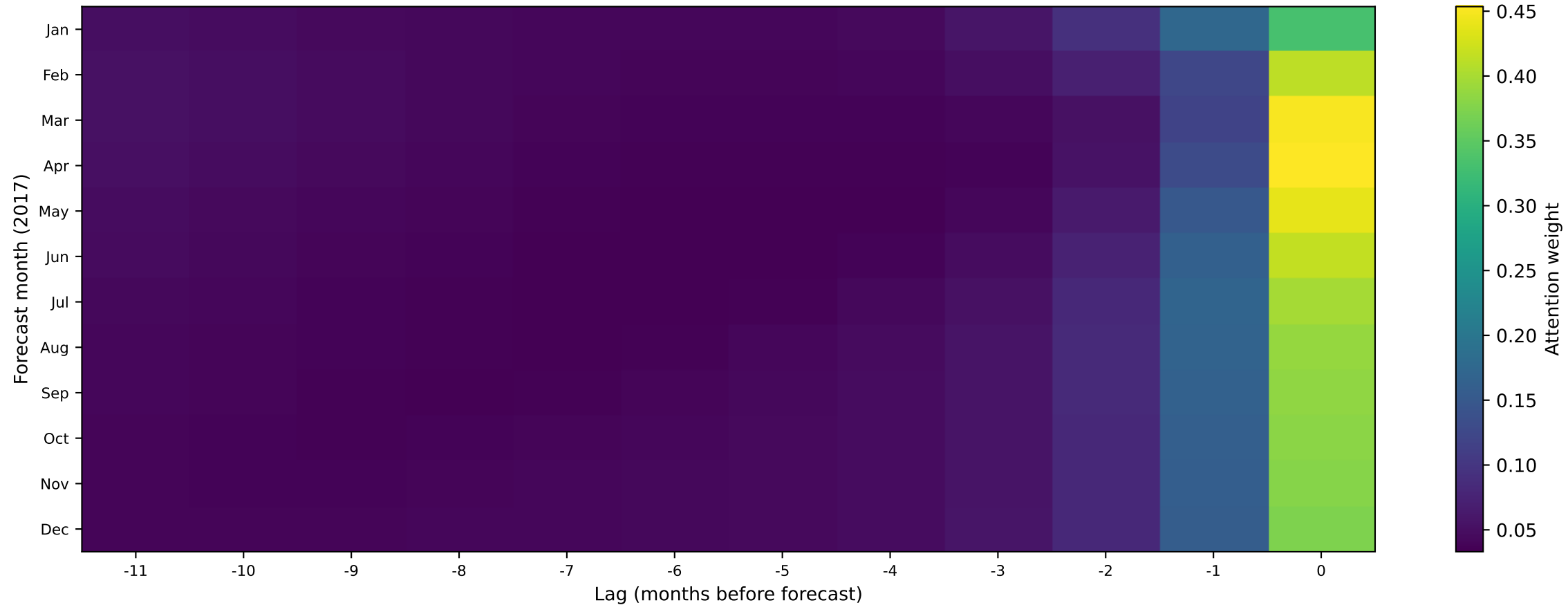
TFT Attention Weights — Electricity Core 2017
