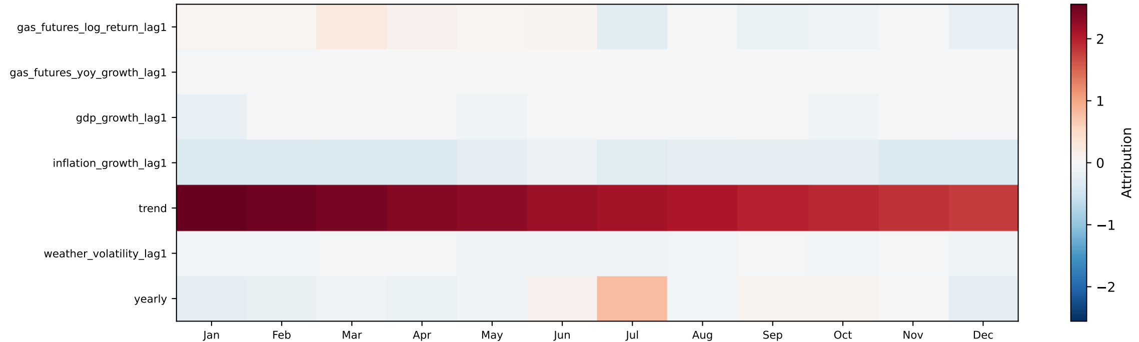
Prophet Component Attribution Heatmap — Gas 2017
