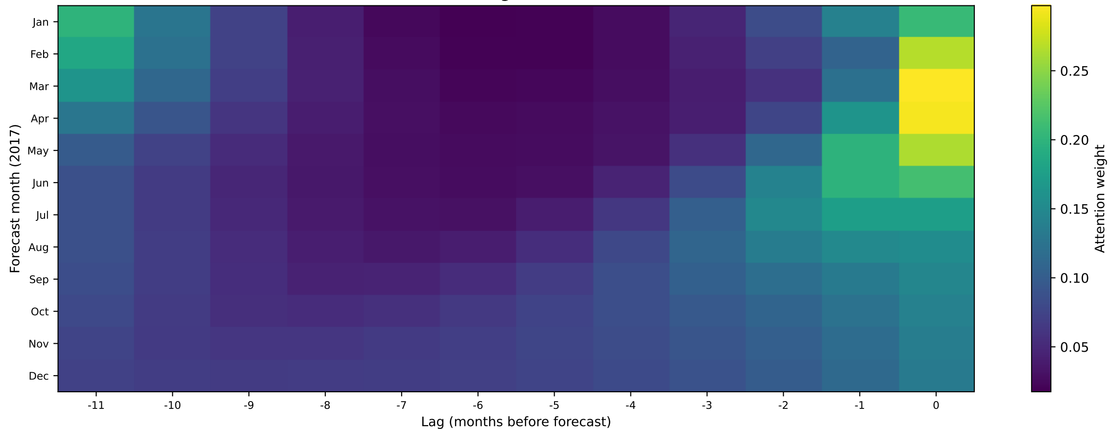
TFT Attention Weights — Gas Core 2017
