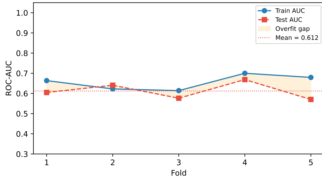
Train vs. Test AUC per CV fold
