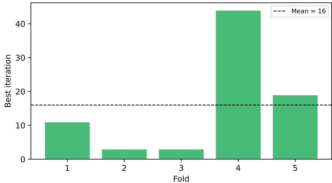
Early stopping iteration per CV fold
