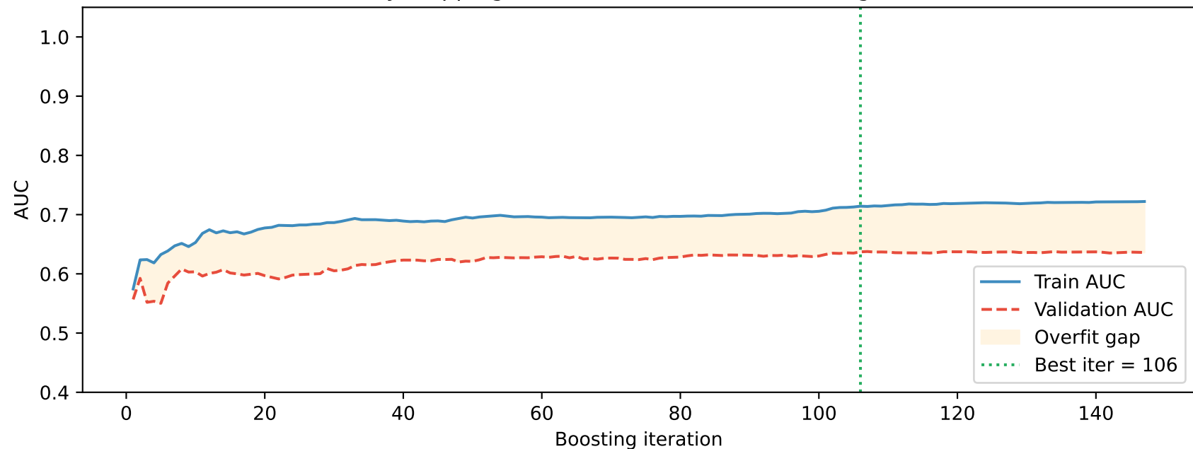
CatBoost learning curve — controls_only (early stopping halts before validation AUC degrades)
