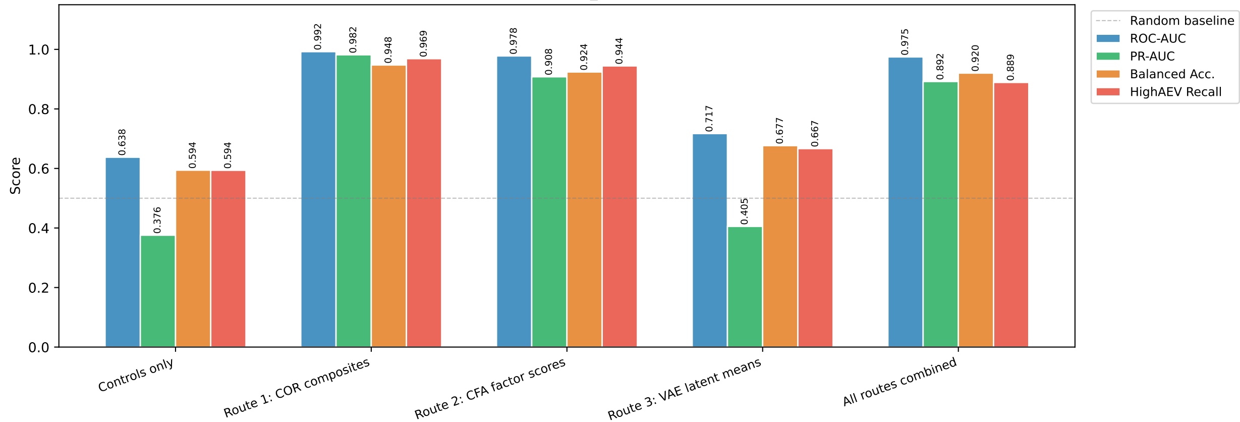
HighAEV classification — feature set comparison (CatBoost, same hyperparameters; Route1_Composite circular by construction)
