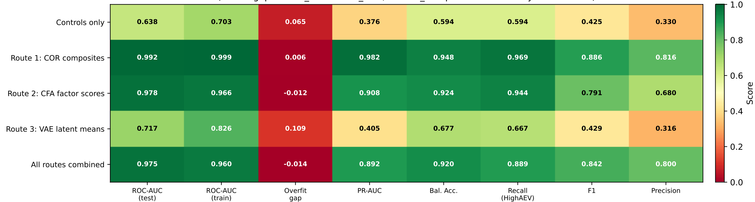
HighAEV classification: model comparison (overfit gap = train_AUC – test_AUC; Route1_Composite is circular by construction)
