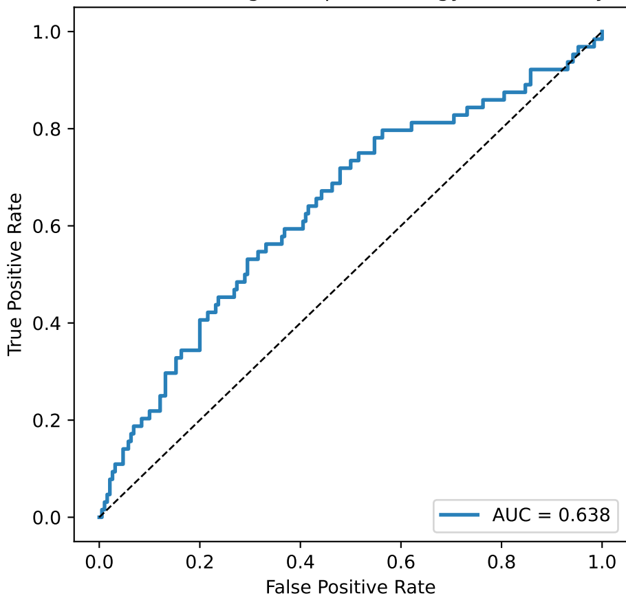
ROC curve: High Adaptive Energy Vulnerability
