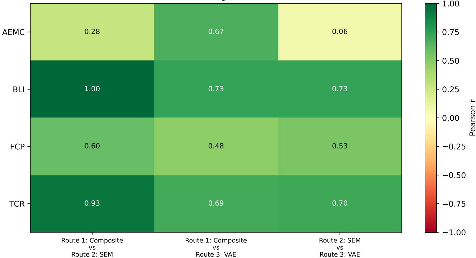
Cross-route construct agreement (Pearson r)
