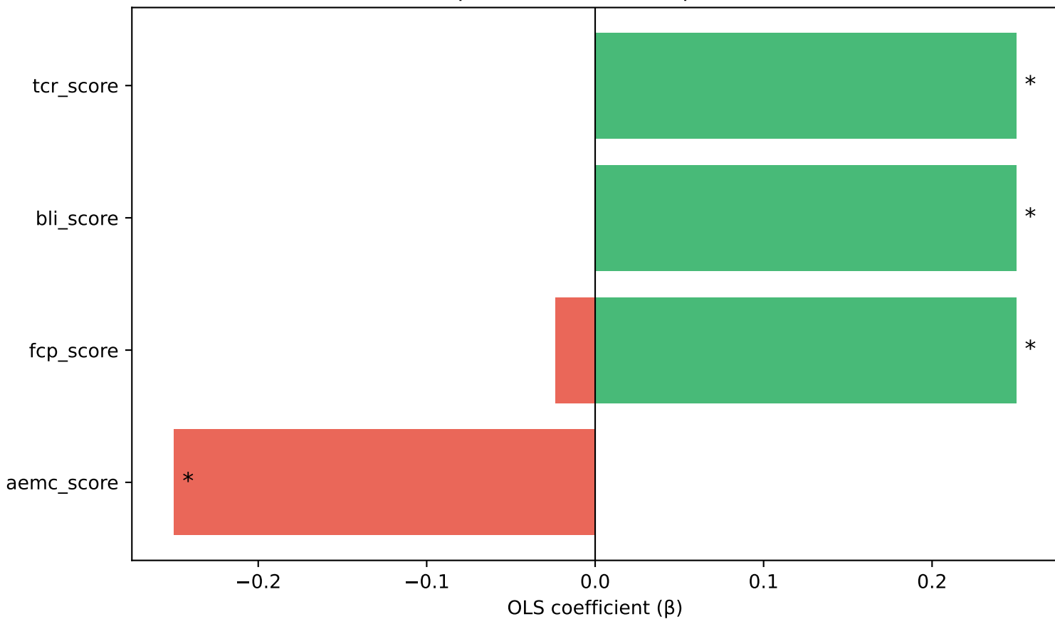
COR path coefficients (* p < 0.05)
