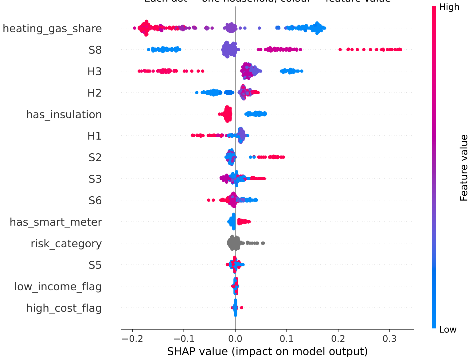
SHAP beeswarm: feature impact on High AEV prediction Each dot = one household; colour = feature value
