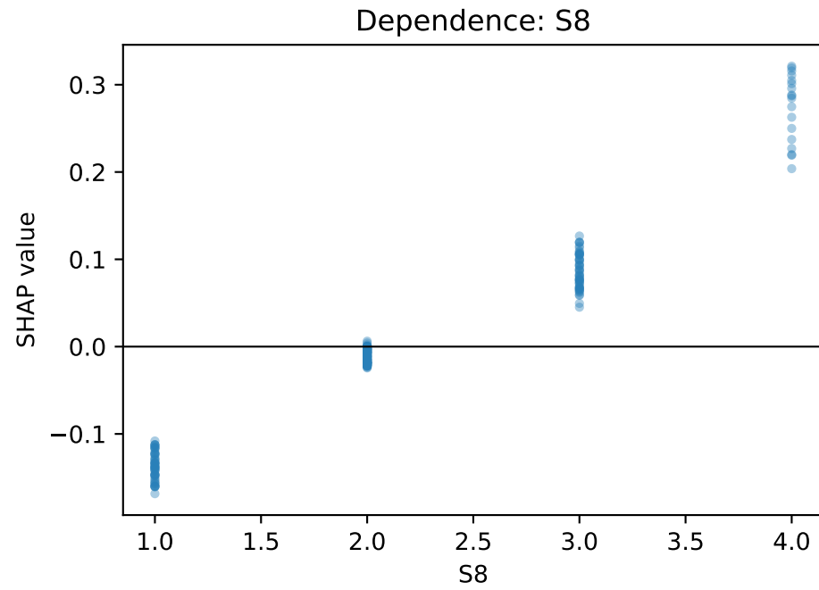
SHAP dependence plots (top features)
