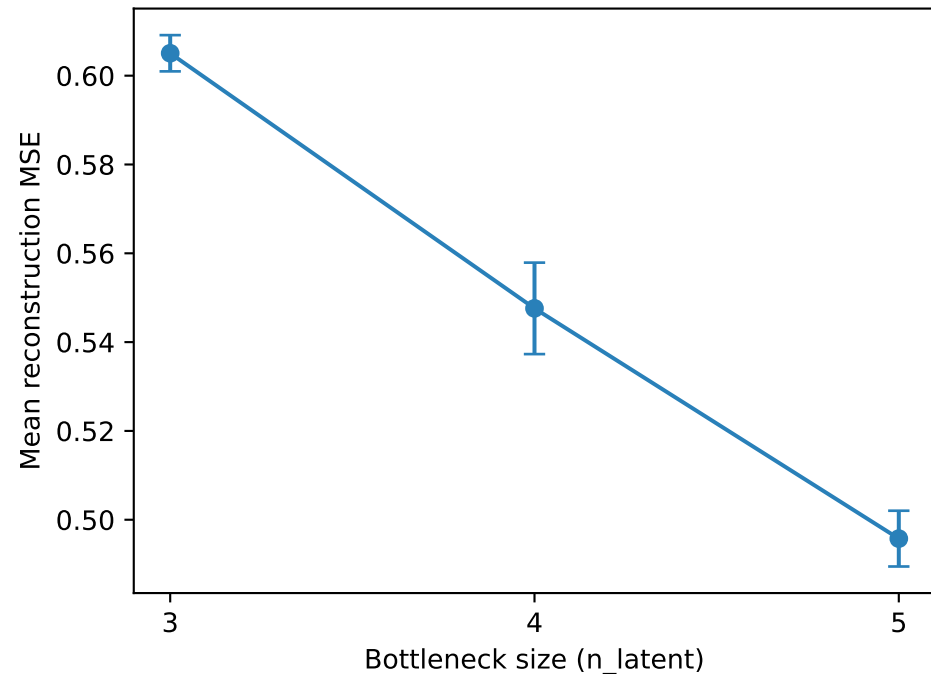
Reconstruction MSE vs bottleneck size
