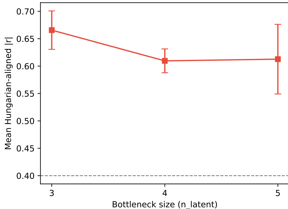
COR alignment quality vs bottleneck size
