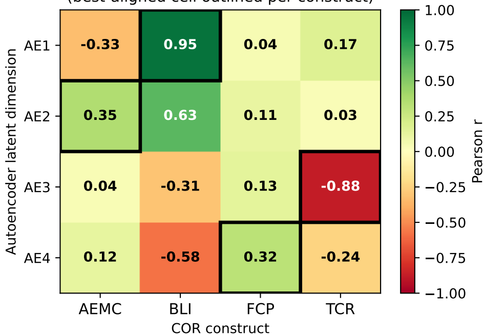
Linear autoencoder latent dims vs. COR construct scores (best-aligned cell outlined per construct)
