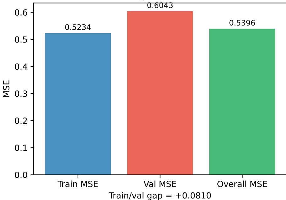
Linear autoencoder reconstruction loss (n_latent=4)
