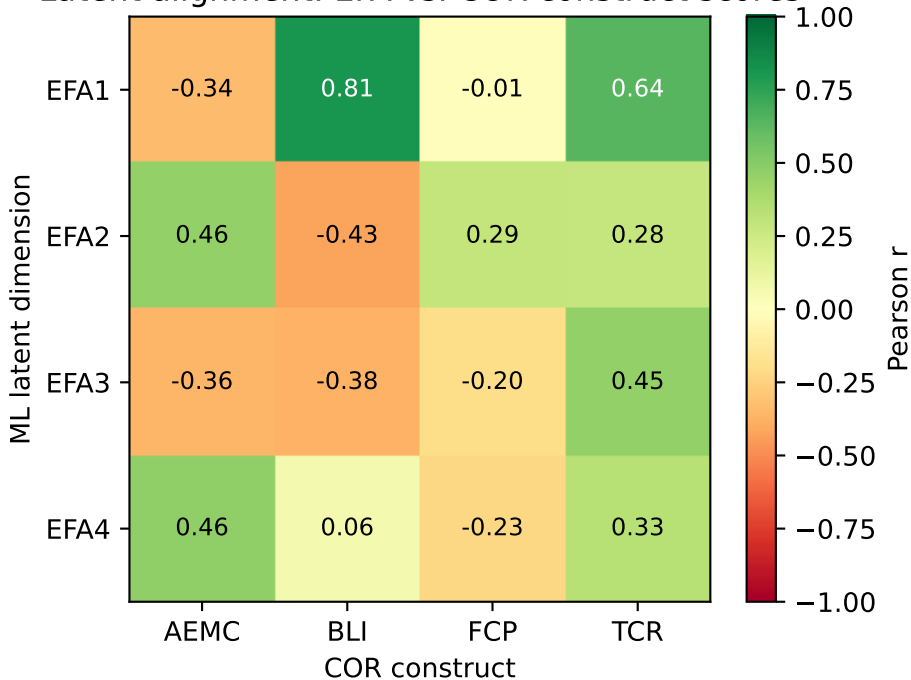
Latent alignment: EFA vs. COR construct scores
