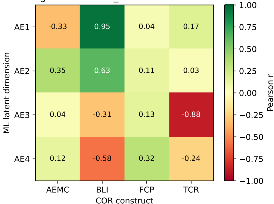
Latent alignment: Linear_AE vs. COR construct scores
