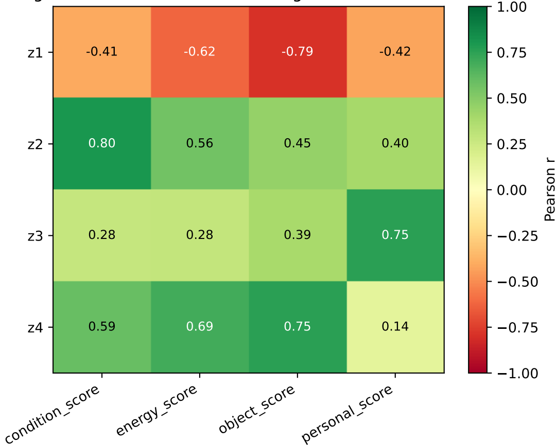
Stage 2c: CVAE latent dims vs. Stage 2b SEM factor scores
