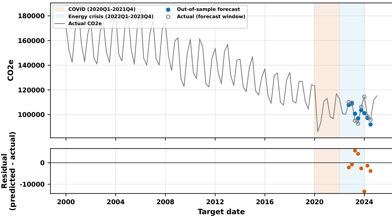
Best_A: A3/all_features/lightgbm, H2 (MASE=0.575, n_features=23)
