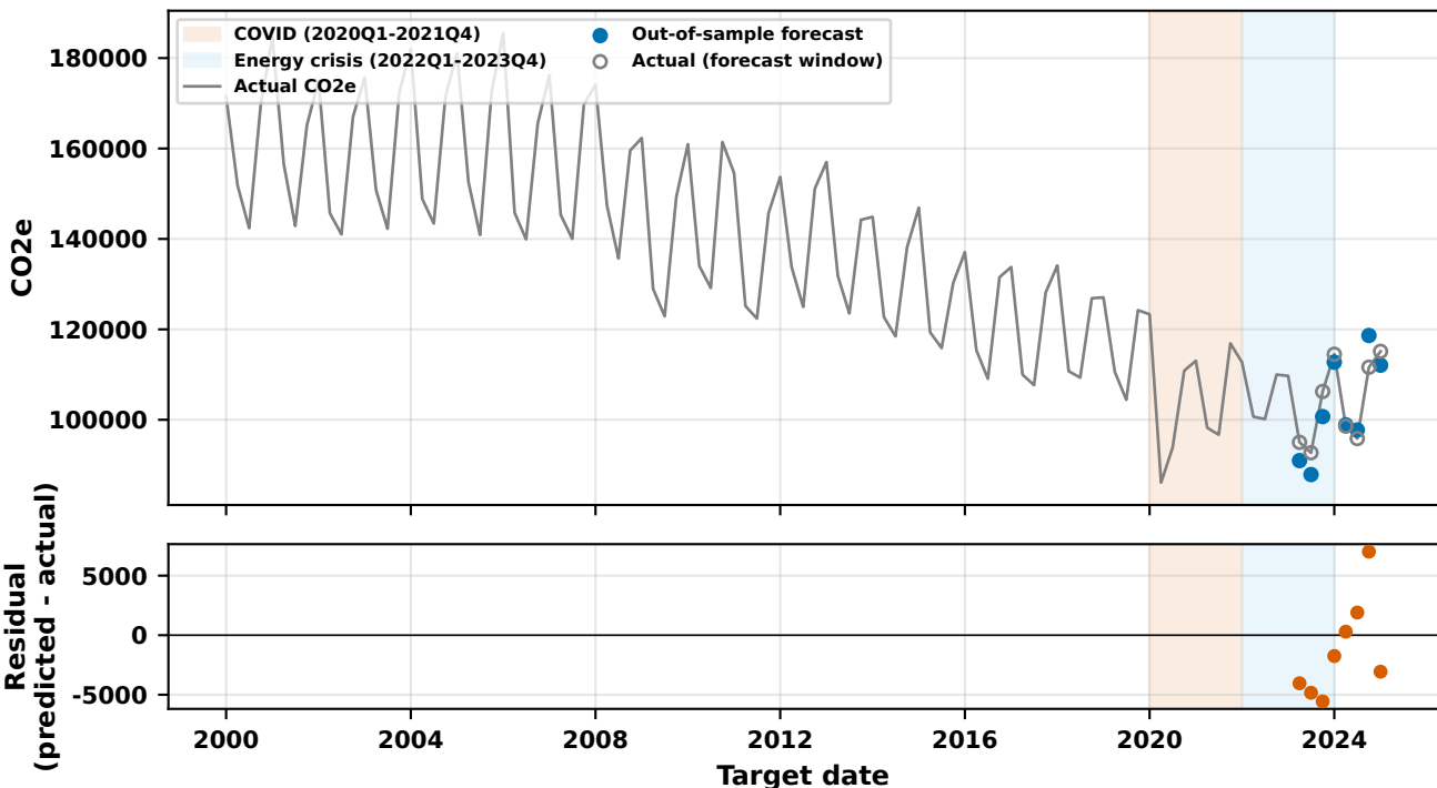
Best_A: A3/all_features/lightgbm, H4 (MASE=0.467, n_features=23)
