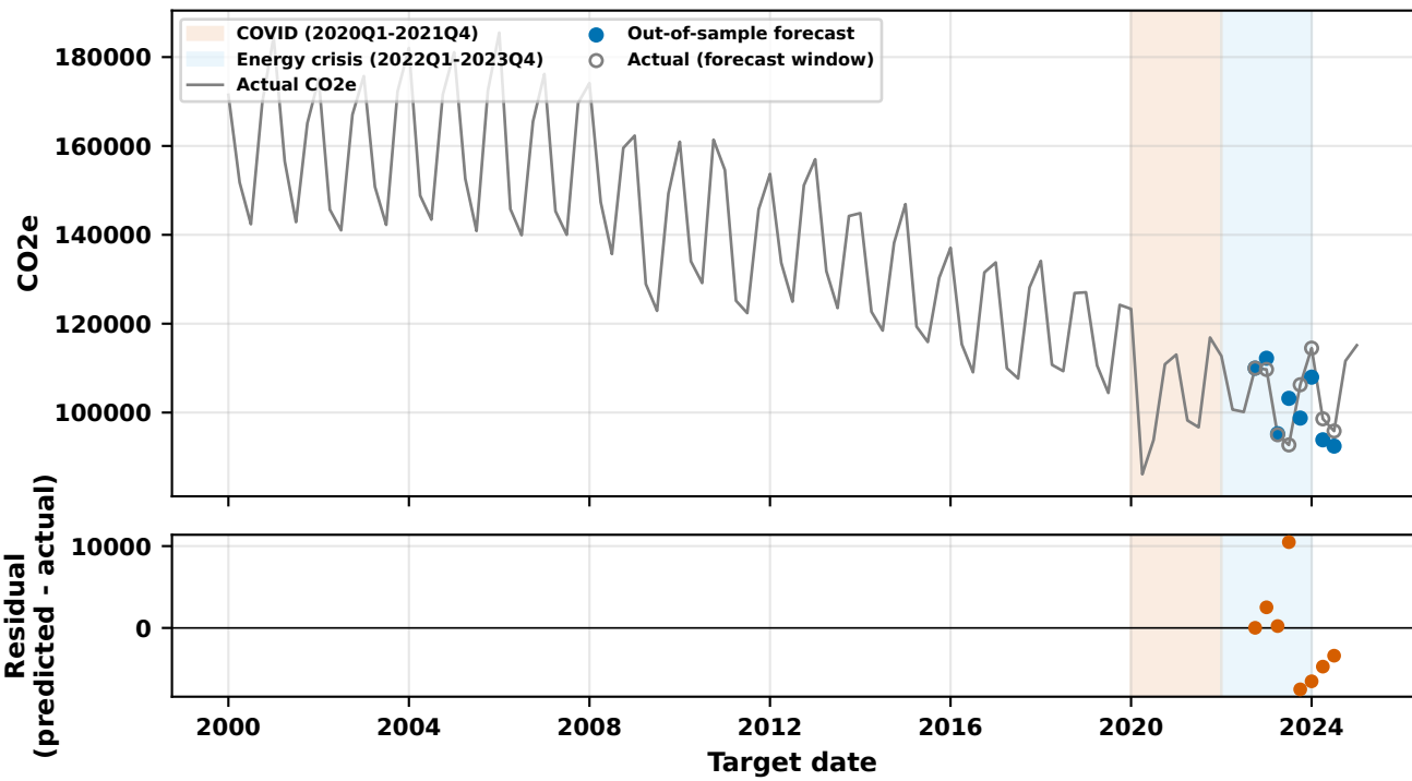
Best_B: A1/fs_linear/catboost, H2 (MASE=0.597, n_features=6)
