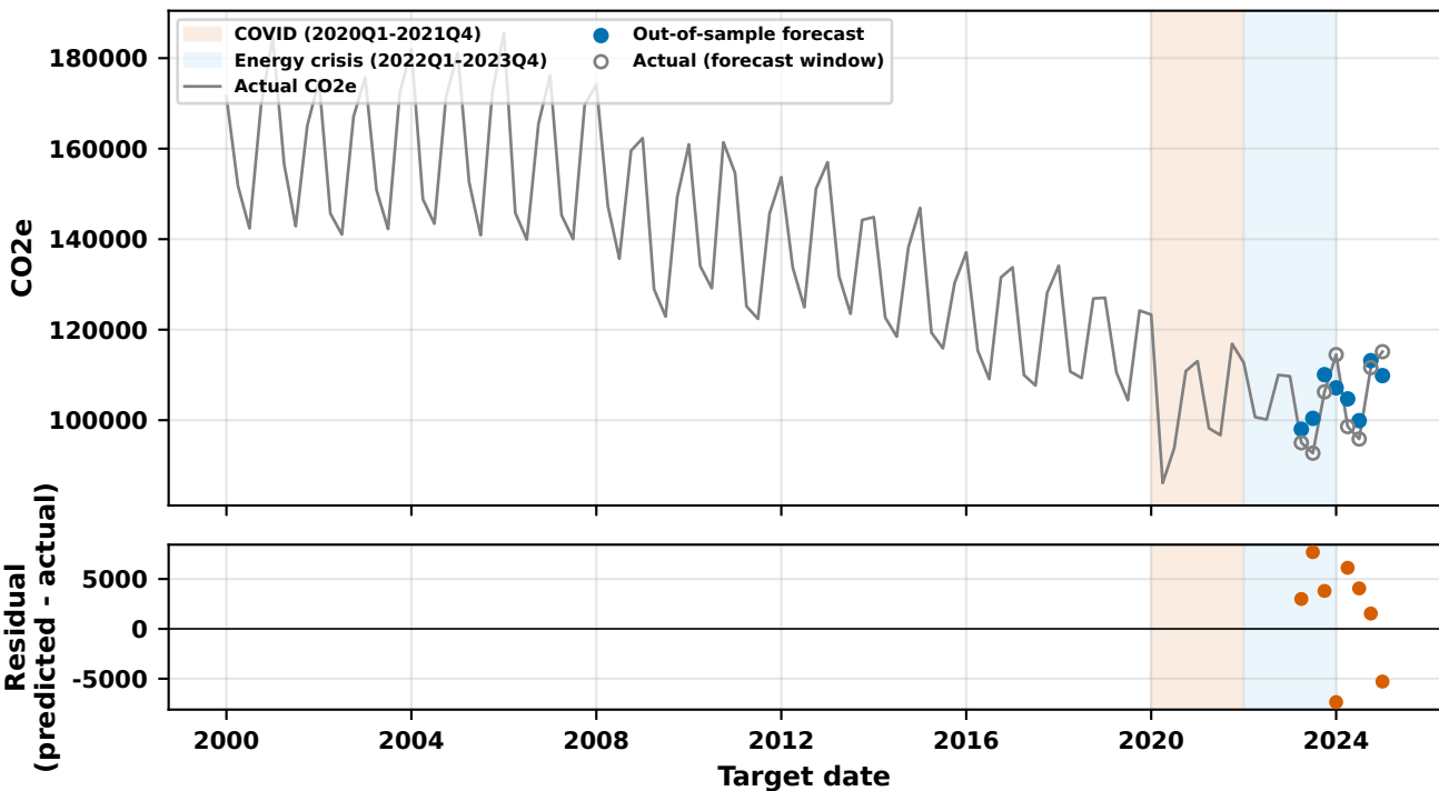
Best_B: A1/fs_linear/catboost, H4 (MASE=0.637, n_features=6)
