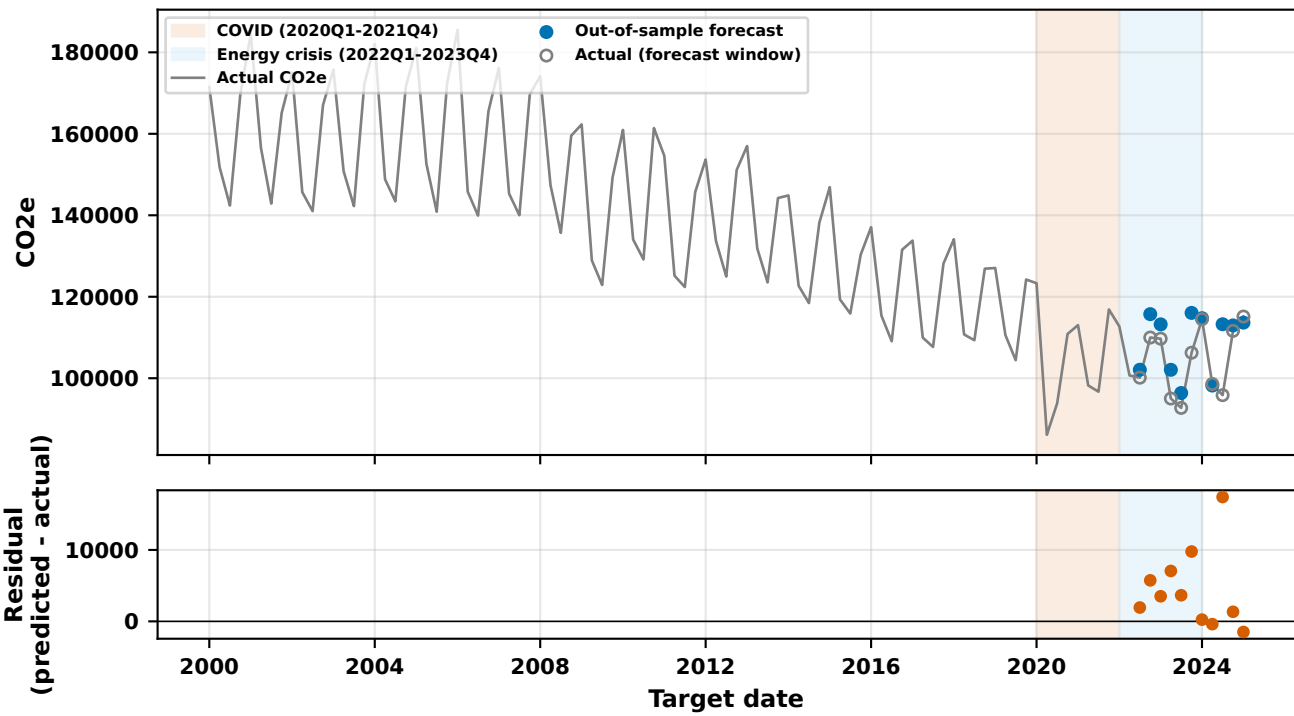
A1 family winner (Stream A): A1/all_features/catboost, H1 (MASE=0.677, n_features=11)
