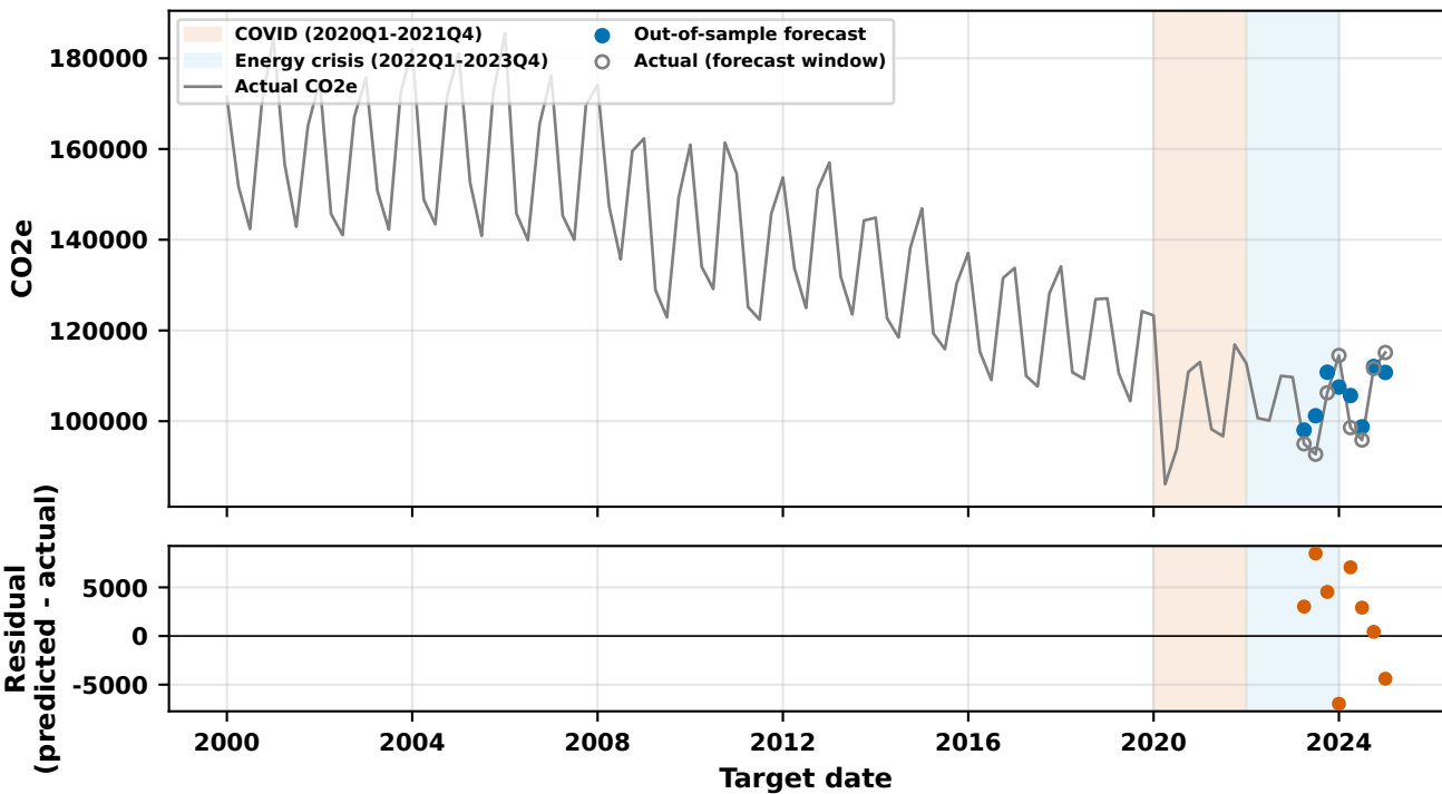
A1 family winner (Stream A): A1/all_features/catboost, H4 (MASE=0.621, n_features=11)
