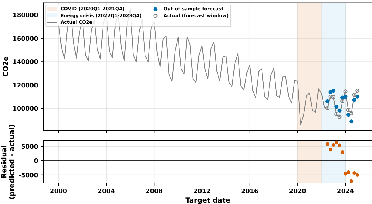
A2 family winner (Stream A): A2/all_features/lstm, H1 (MASE=0.711, n_features=25)
