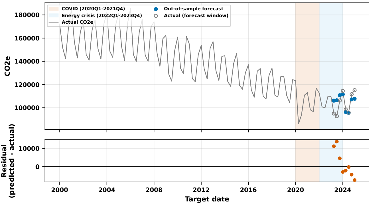
A2 family winner (Stream A): A2/all_features/lstm, H4 (MASE=0.765, n_features=25)
