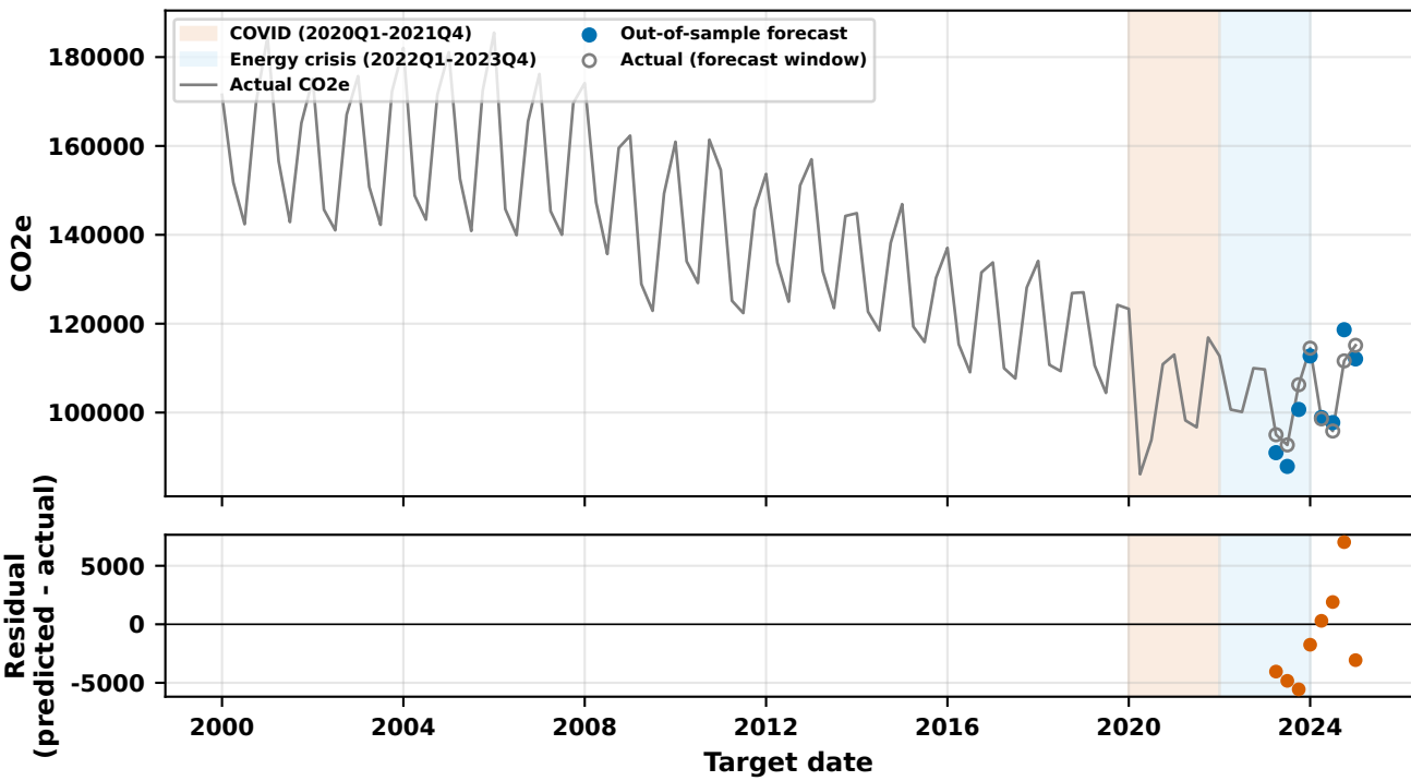
A3 family winner (Stream A): A3/all_features/lightgbm, H4 (MASE=0.467, n_features=23)
