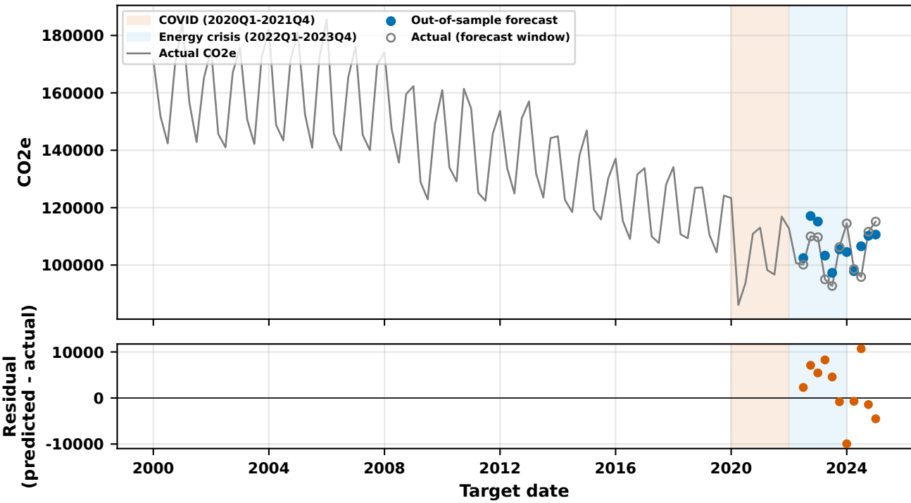
A4 family winner (Stream A): A4/all_features/catboost, H1 (MASE=0.719, n_features=37)
