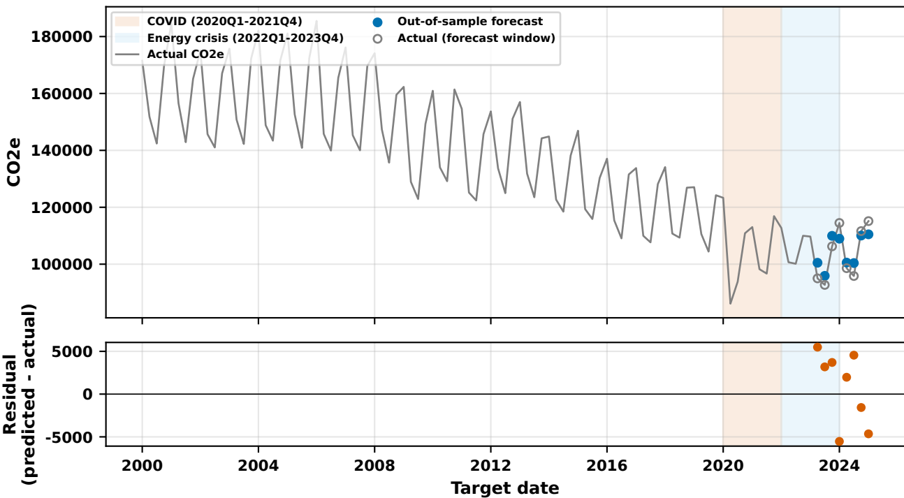
A4 family winner (Stream A): A4/all_features/catboost, H4 (MASE=0.503, n_features=37)
