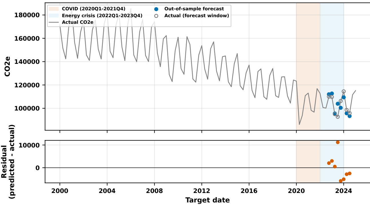
B1 family winner (Stream B): A1/fs_wrapper/catboost, H2 (MASE=0.556, n_features=11)
