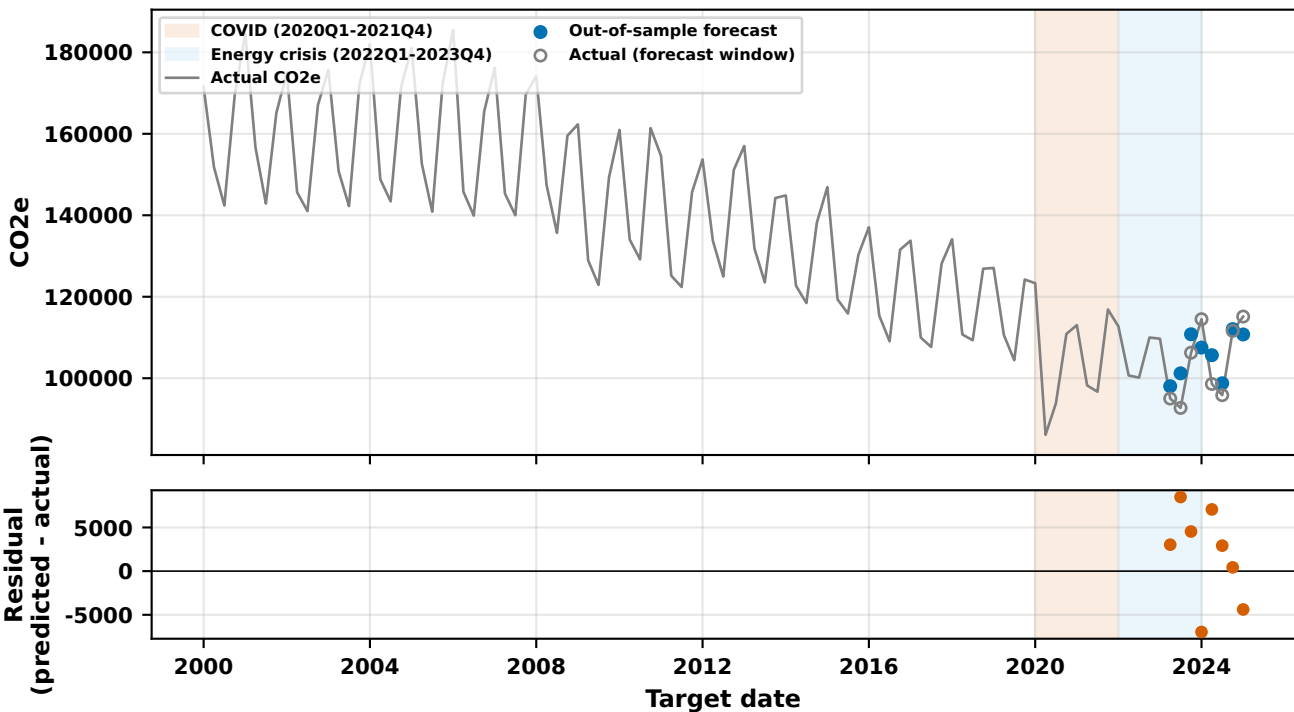
B1 family winner (Stream B): A1/fs_wrapper/catboost, H4 (MASE=0.621, n_features=11)
