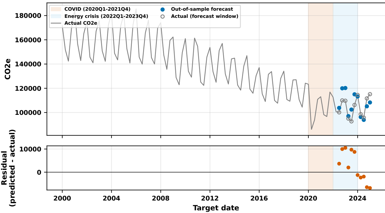
B2 family winner (Stream B): A2/fs_linear/lstm, H1 (MASE=0.817, n_features=11)
