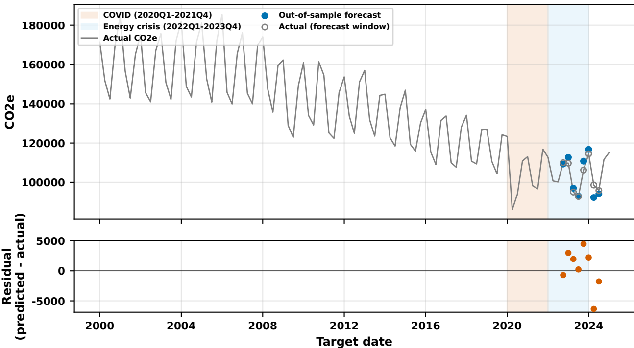
B2 family winner (Stream B): A2/fs_linear/lstm, H2 (MASE=0.350, n_features=11)
