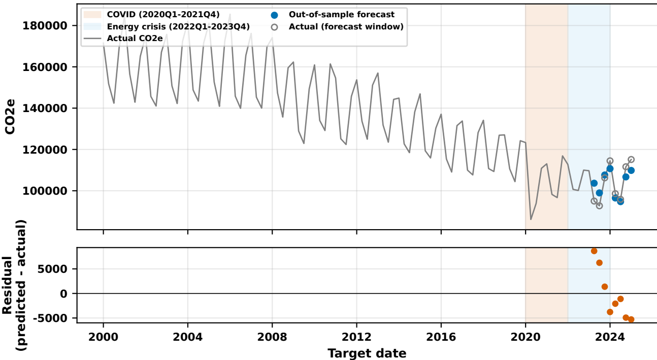
B2 family winner (Stream B): A2/fs_linear/lstm, H4 (MASE=0.549, n_features=11)
