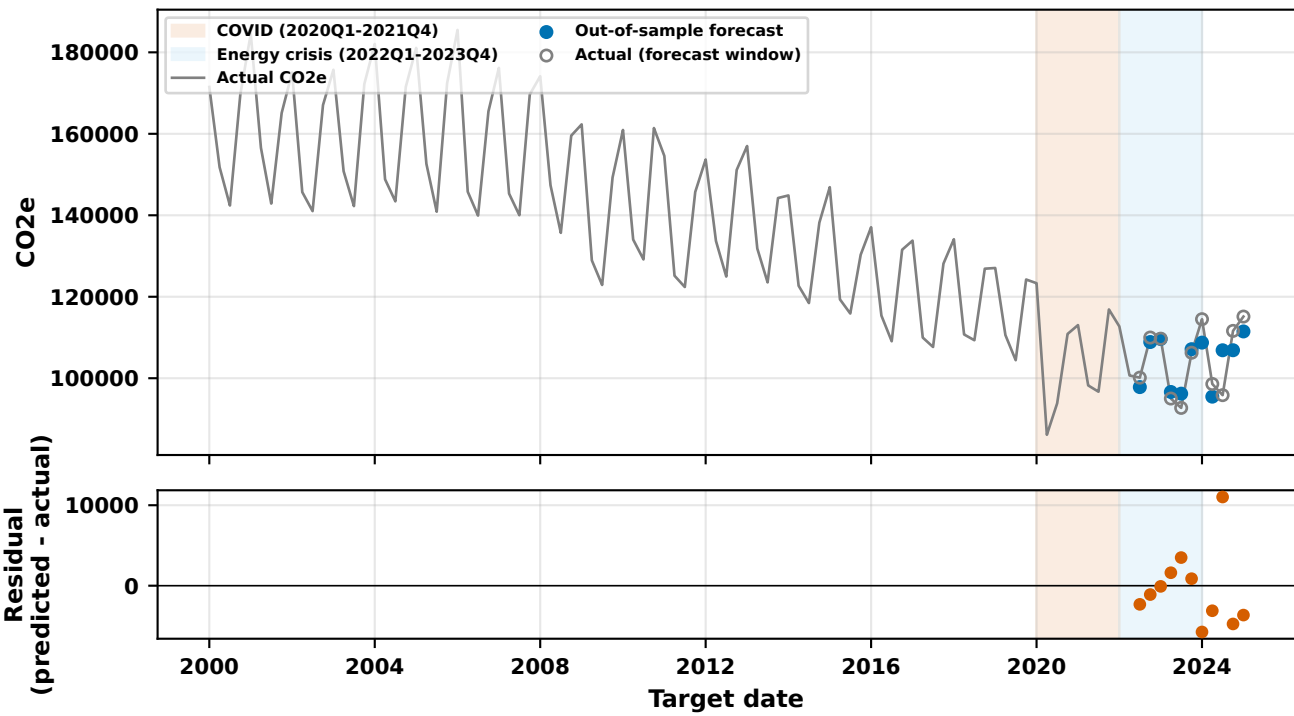
B3 family winner (Stream B): A3/fs_wrapper/lightgbm, H1 (MASE=0.486, n_features=15)
