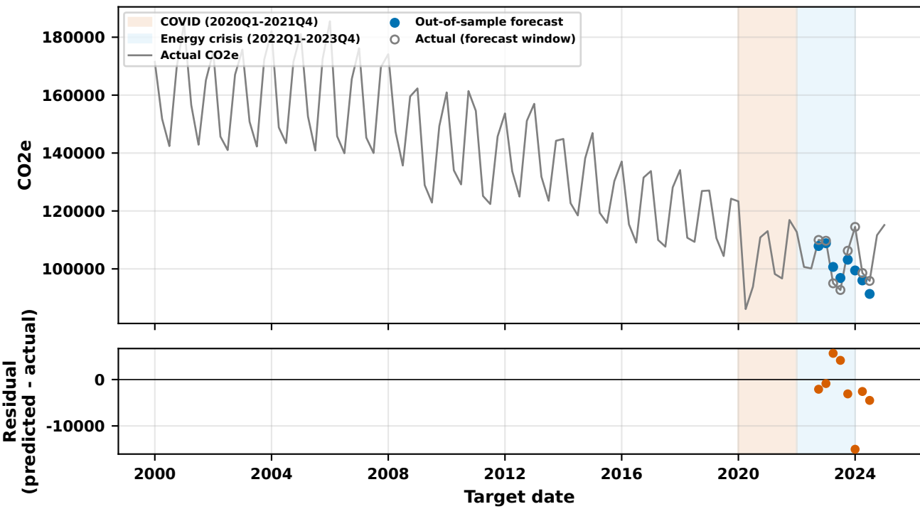
B3 family winner (Stream B): A3/fs_wrapper/lightgbm, H2 (MASE=0.640, n_features=15)
