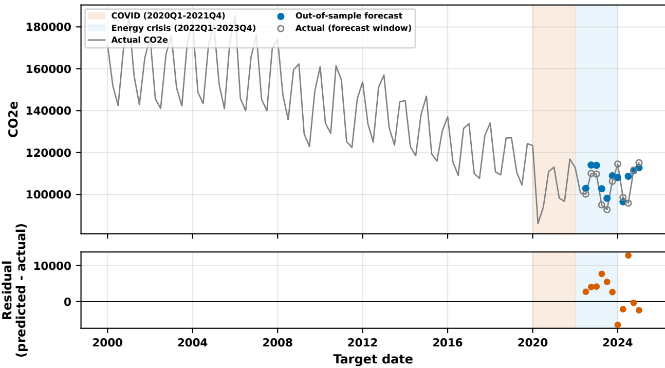
B4 family winner (Stream B): A4/fs_wrapper/catboost, H1 (MASE=0.654, n_features=21)
