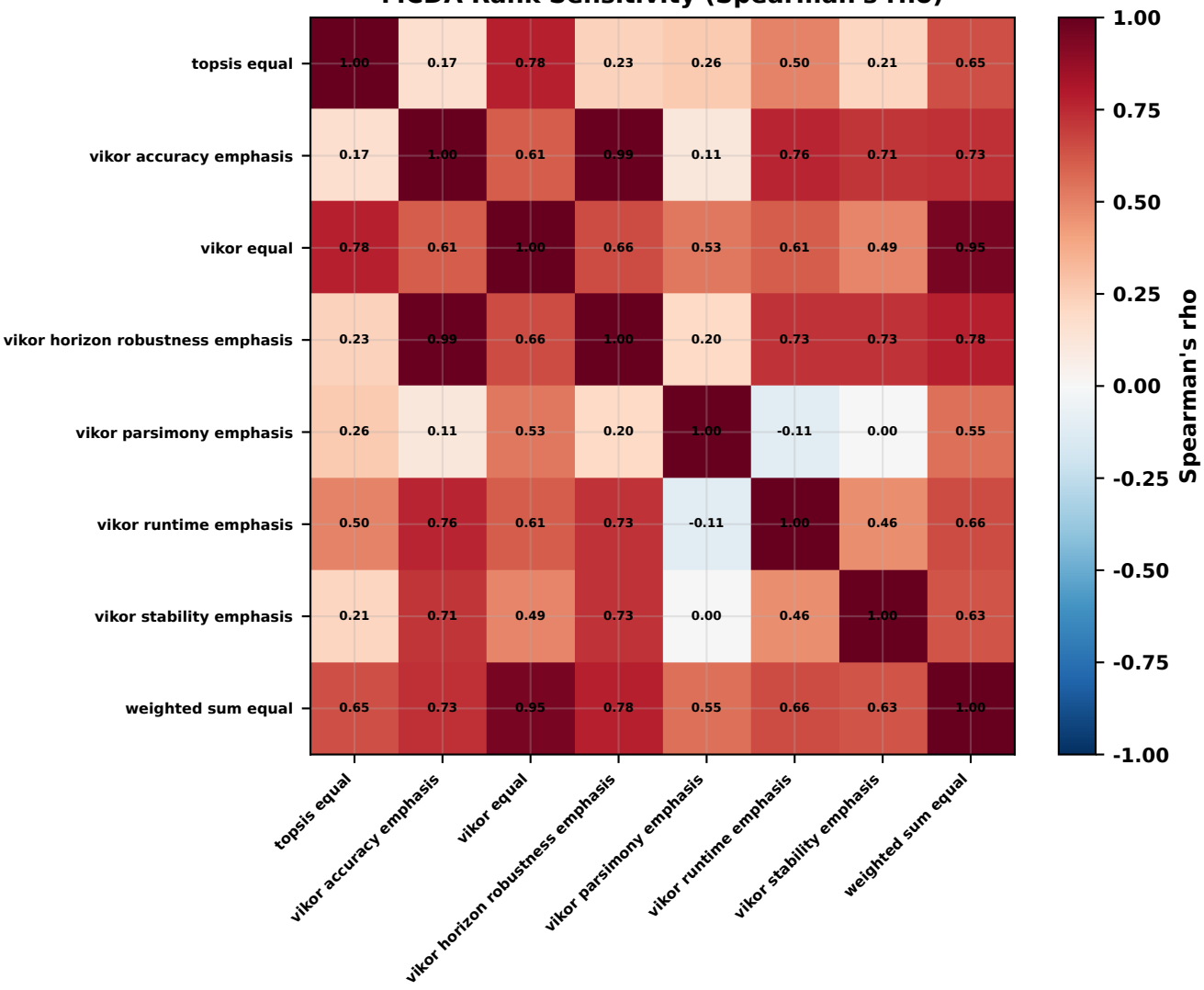
MCDA Rank Sensitivity (Spearman's rho)
