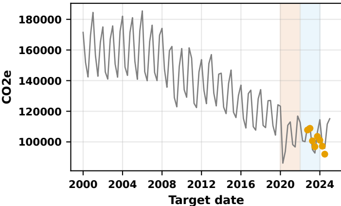
Best_A: A3/all_features/lightgbm MASE=0.575
