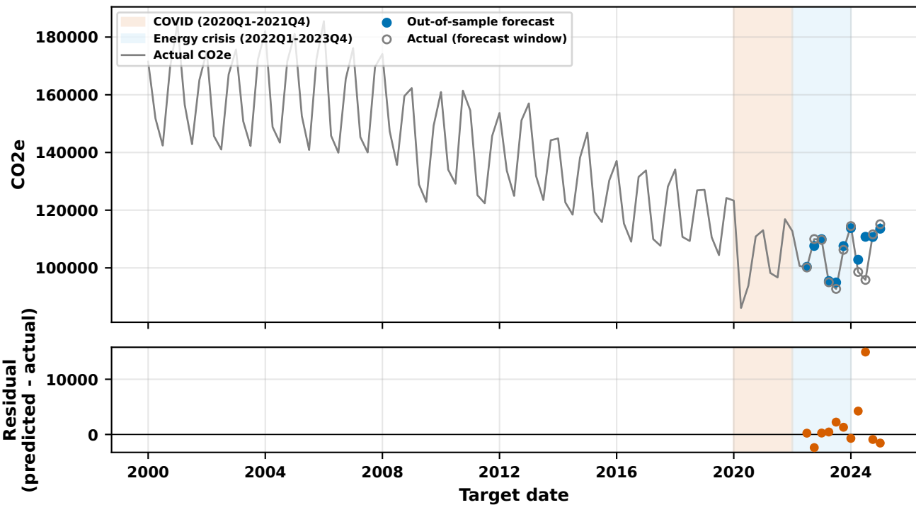
Best_Overall: A3/all_features/lightgbm, H1 (MASE=0.376, n_features=23)
