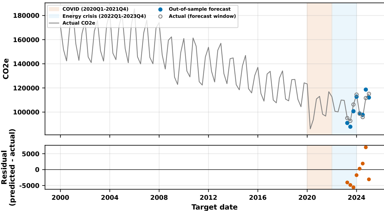
Best_Overall: A3/all_features/lightgbm, H4 (MASE=0.467, n_features=23)
