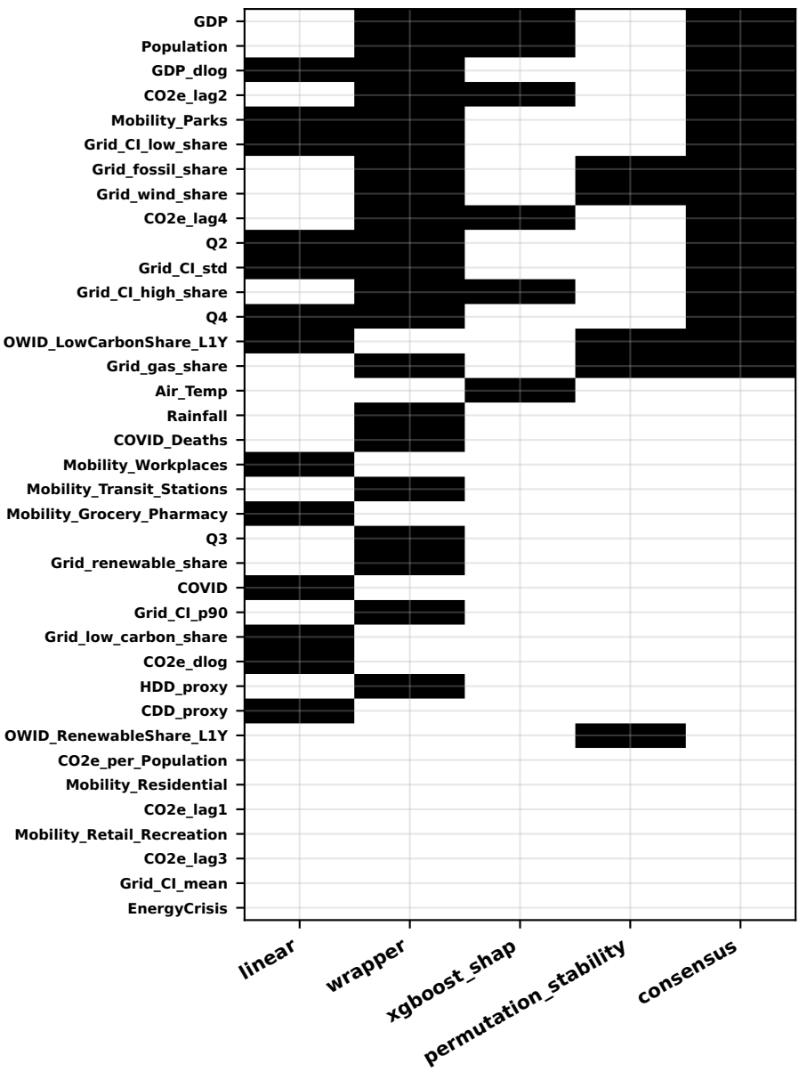
B4: Feature-Selection Membership
