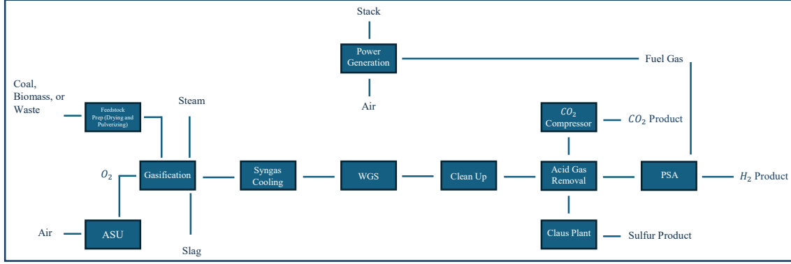
Figure 1: Process flow diagram for biomass gasification to hydrogen production, showing feedstock preparation, gasification, syngas cleanup, CO 2 management, hydrogen separation, and energy integration.
