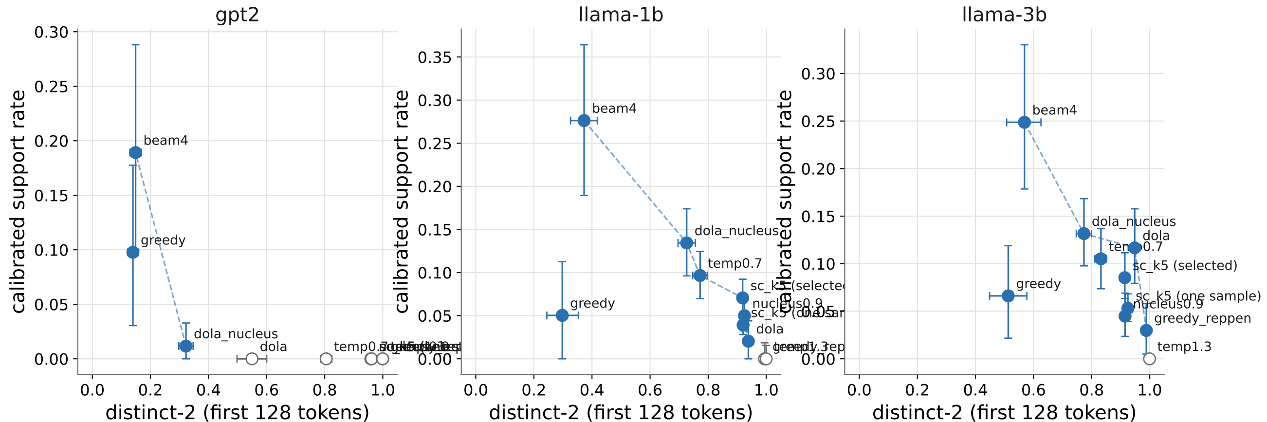
Factuality against diversity, by model scale (hollow = calibrates to zero)
