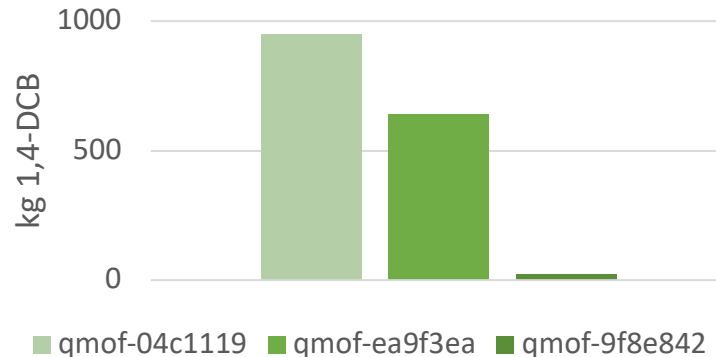
Marine Ecotoxicity
