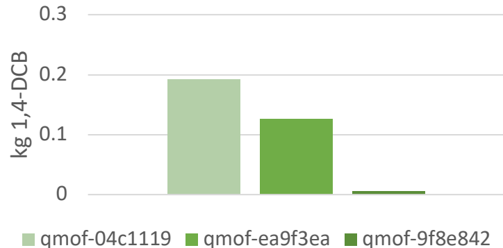
Freshwater Ecotoxicity
