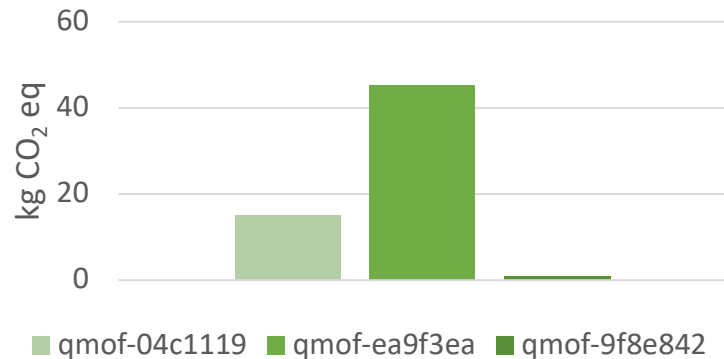
Global Warming
