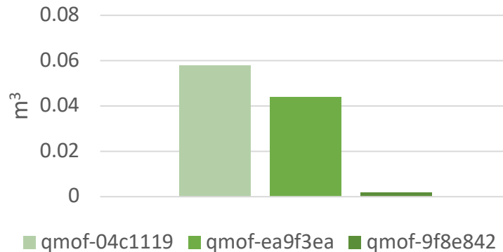
Water Consumption
