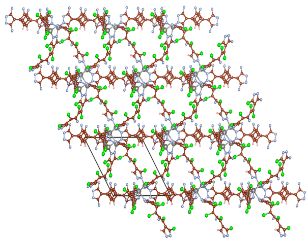
qmof-74ace65
