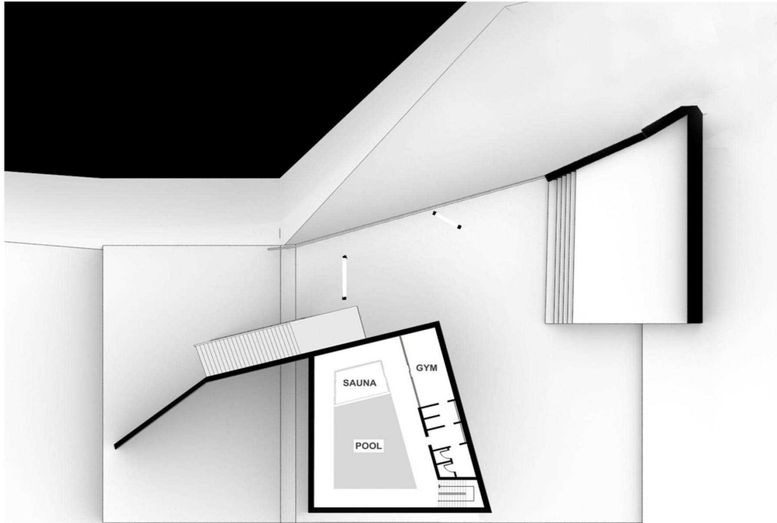
BASEMENT
