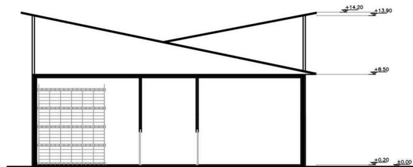
C-C SECTION
